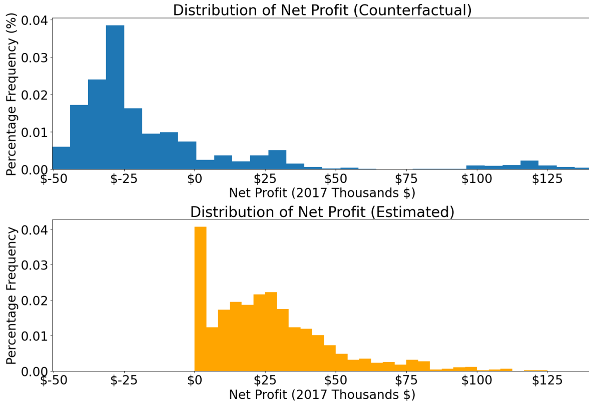
Figure 18: Counterfactual Expected Profit - Popular Recommendations
